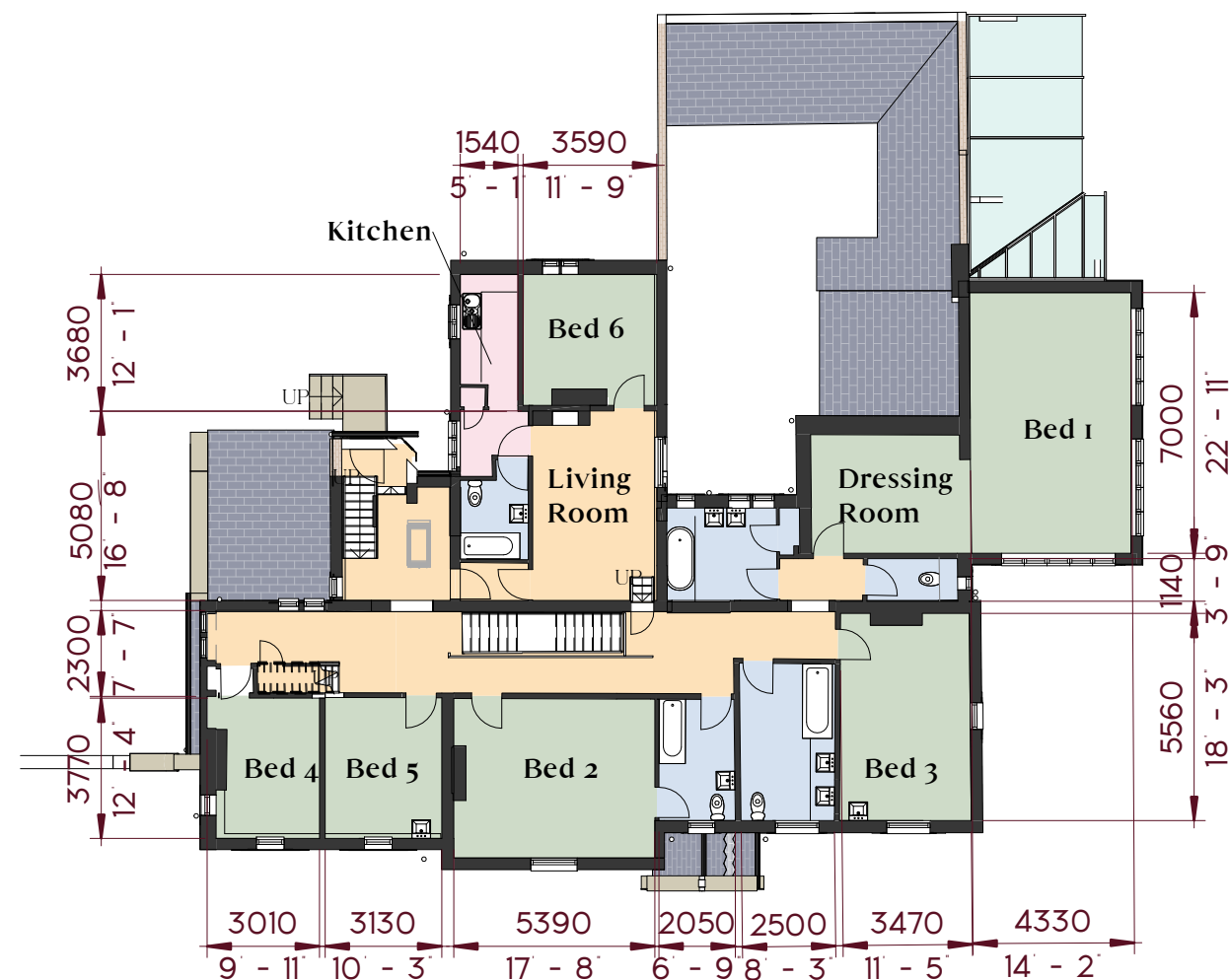
Main House - Existing First Floor
